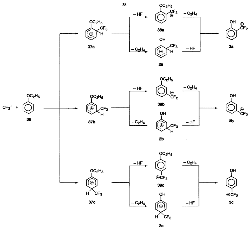
Scheme 13.
